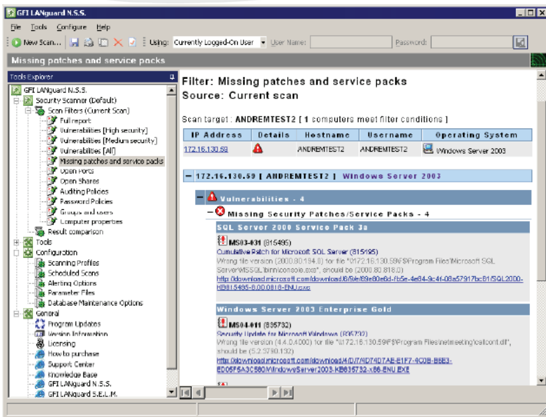
The GFI LANguard missing patches/service packs report
